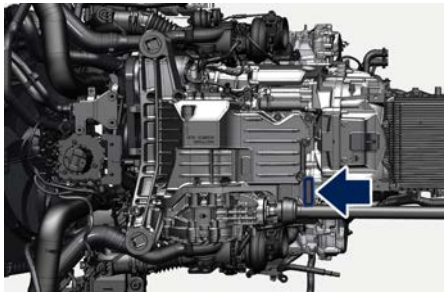
3.8 V8 - Engine
